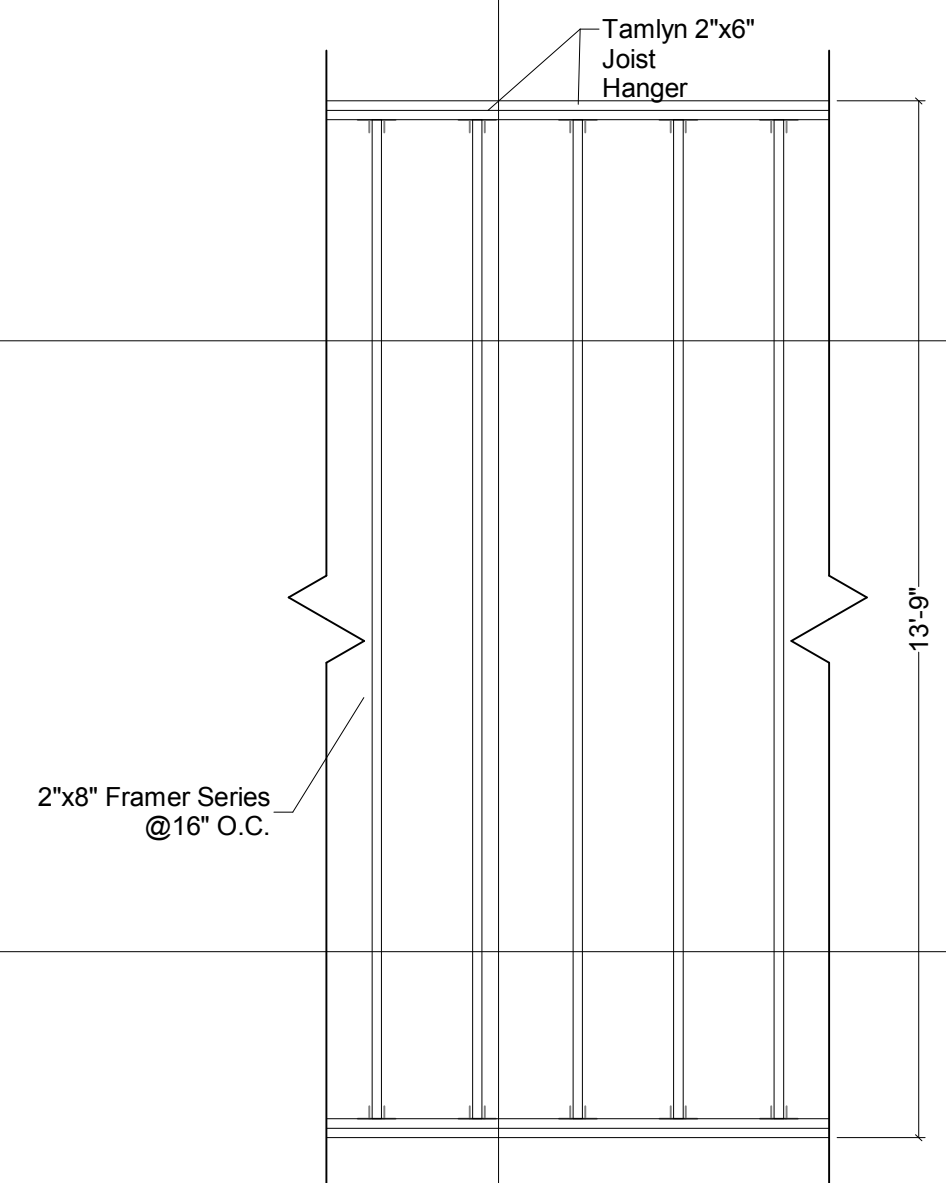
Floor Joist Detail
