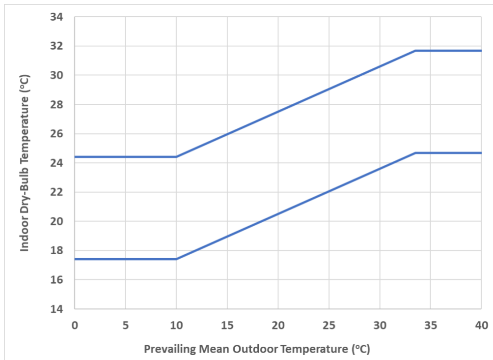
Figure 1. Adaptive Comfort Range Based on Prevailing Mean Outdoor Temperature
